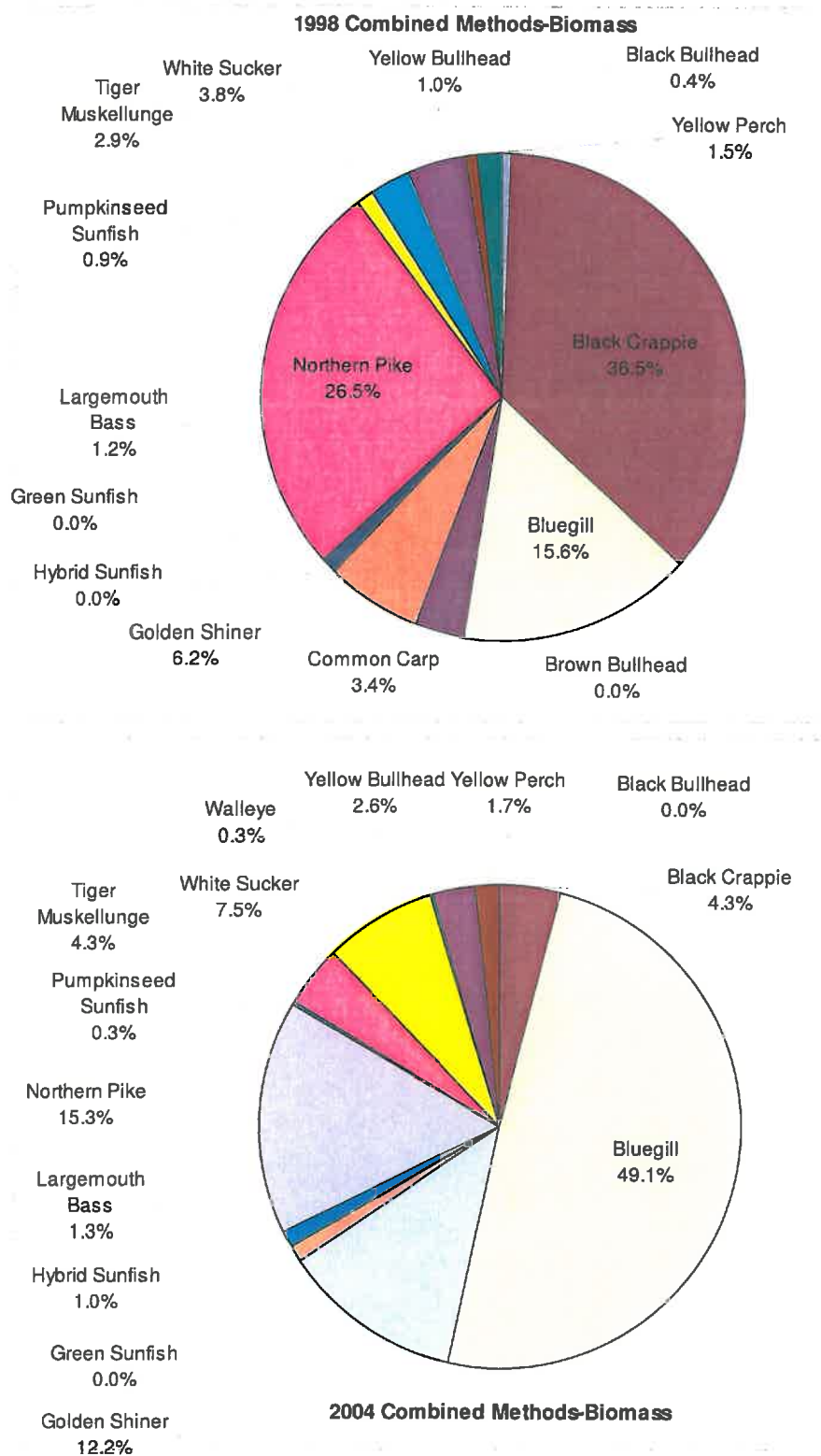
Figure 3.7. 1998 and 2004 fish survey results for total fish biomass in Crystal Lake.
