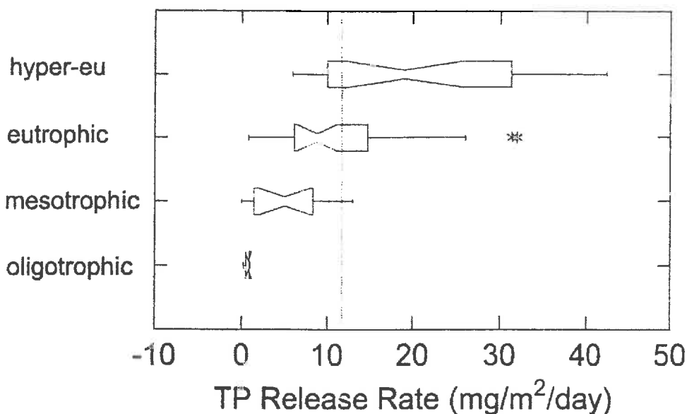
Figure 6.1. Sediment phosphorus release rates by trophic condition. (Nürnberg 1997)
